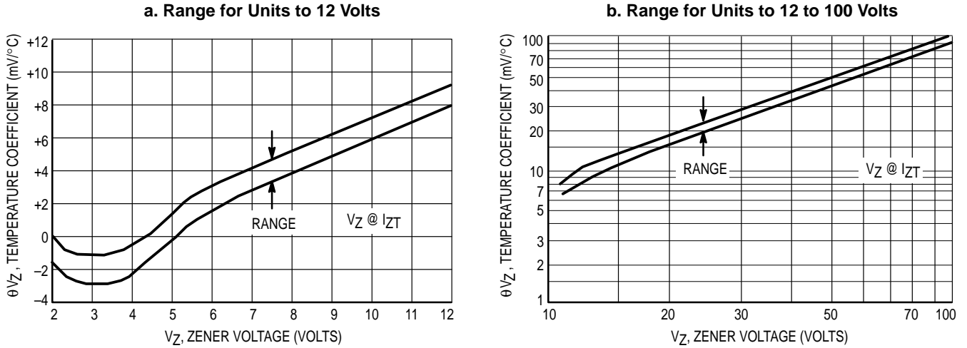
Figure 2. Temperature Coefficients
